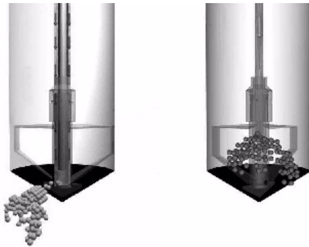
Figure 1. Principle of the MDM process. Example of mixing tool. (Left) A predetermined amount of water is added through conduits to alter liquidity index, water content or water/binder ratio. (Right) Binder is added through separate conduits, in amounts corresponding to modified amounts of available water.
