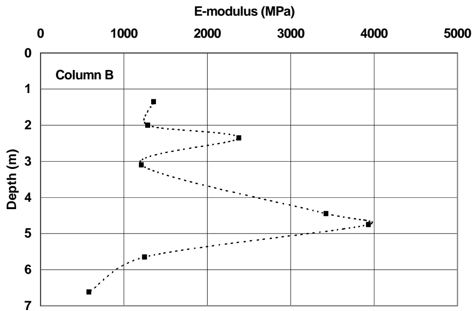
Figure 7. E50-modulus in MDM column B, Tullinge.
