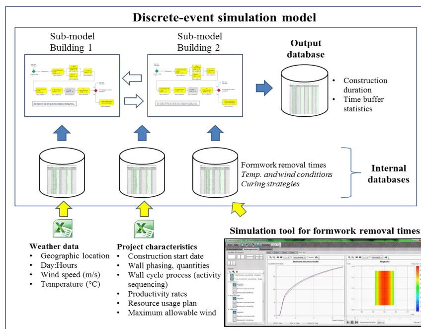
Fig. 2. Overview of discrete-event simulation model.
