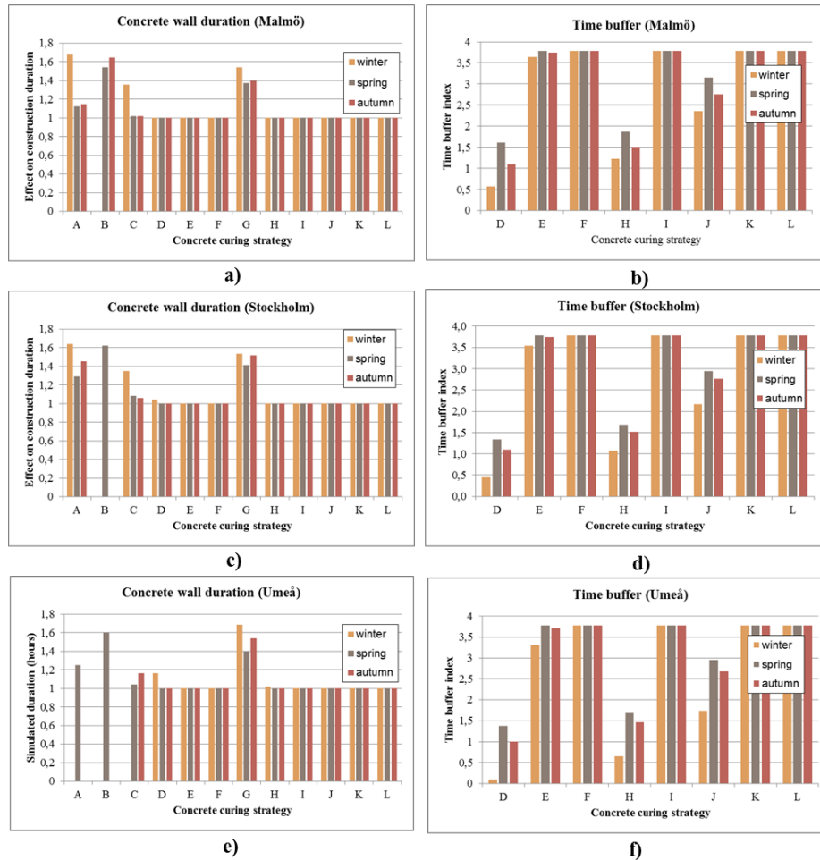
Fig. 4. Simulated effect on construction duration for various seasons and geographical locations (diagrams a, c and e). Diagrams b, d and f show corresponding time buffer index.
