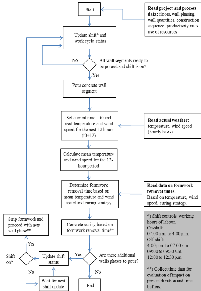
Fig. 3. Outline of the algorithm for estimating formwork removal time based on current weather and selected curing strategy.
