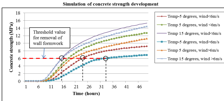
Fig. 1. Estimation of concrete strength and formwork removal times for climatic conditions.
