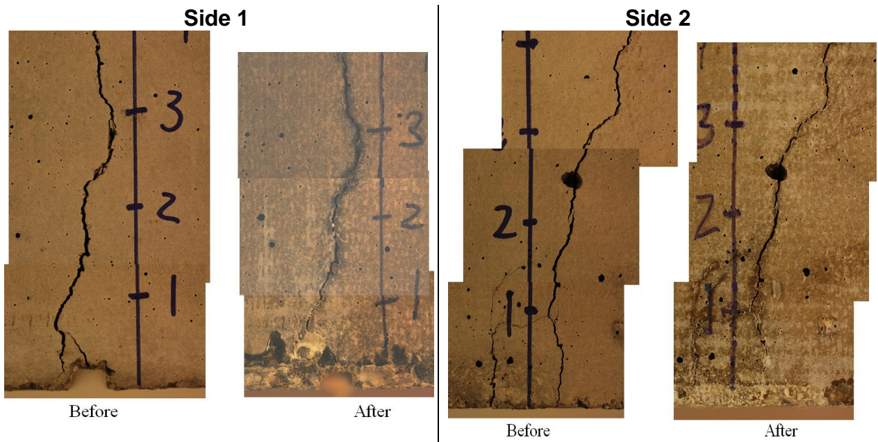
Figure A1.3: Permanently in sea water. Crack width 0.4 mm. Cover 55 mm. Specimen H55-4-1-1
